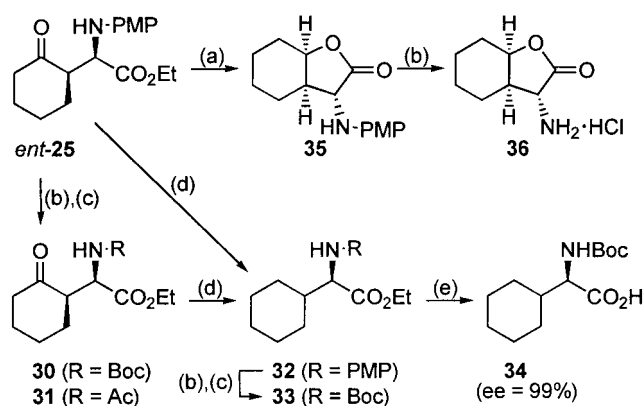
Scheme 1. Synthesis of N -Boc-cyclohexylglycine 34 and \alpha -amino- \delta -lactone 36 . Reagents and conditions: (a) L -Selectride, THF, -78^\circ\text{C} , 89%; (b) \text{PhI}(\text{OAc})_2 , MeOH, 0^\circ\text{C} , 30 min; 1 N HCl, 0^\circ\text{C} , 30 min; (c) aqueous \text{Na}_2\text{CO}_3 , \text{Ac}_2\text{O} (64%) or \text{Boc}_2\text{O} (68%); (d) \text{TsNHNH}_2 , MeOH, \Delta ; then \text{NaBH}_4 , 0^\circ\text{C} \rightarrow \Delta , 50% overall; (e) \text{LiOH} , dioxane/ \text{H}_2\text{O} , r.t., 14 h, 78%.
